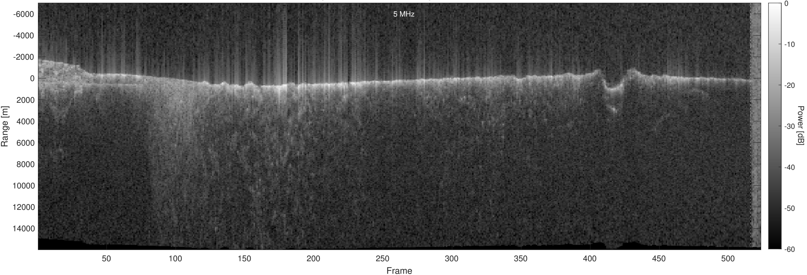
Orbit 16007, Optimized, No Window, Depth-Corrected, Channel 2
