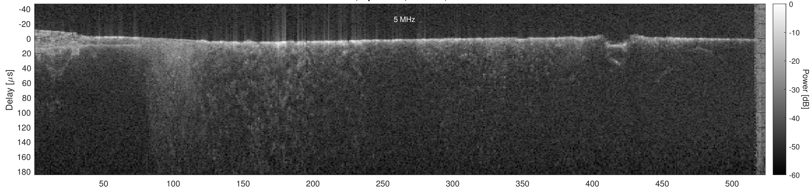
Orbit 16007, Optimized, Window, Channel 2
