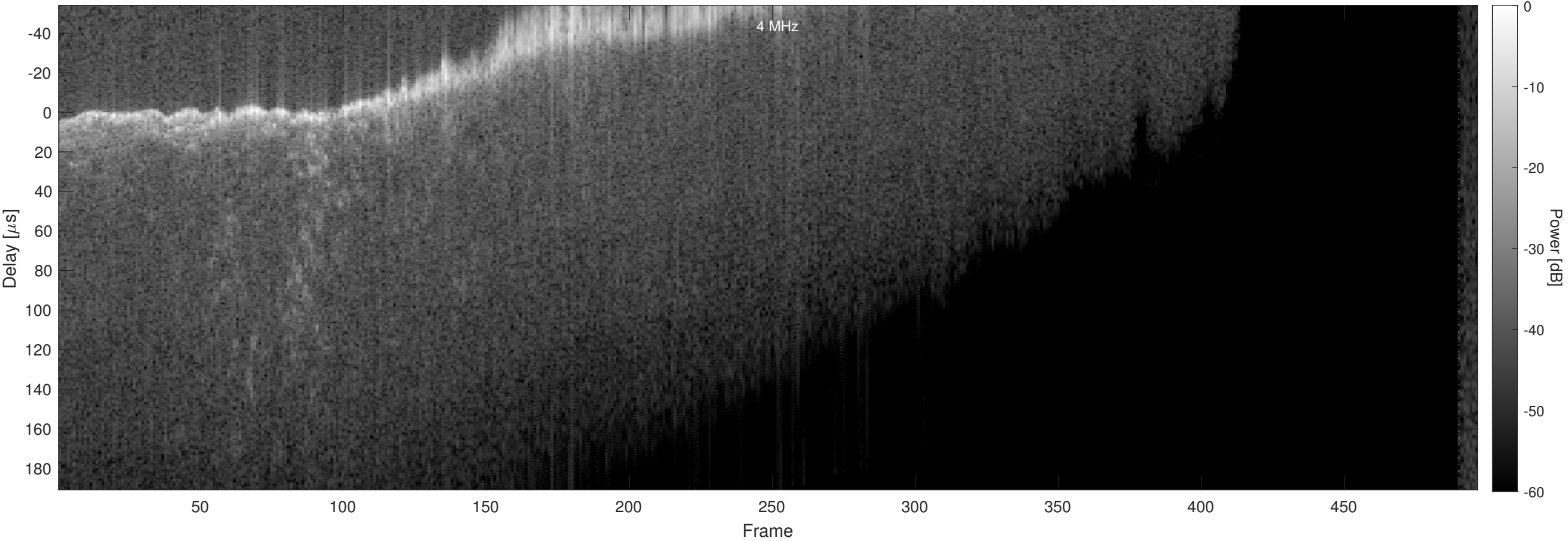
Orbit 16010, Chapman, No Window, Channel 2
