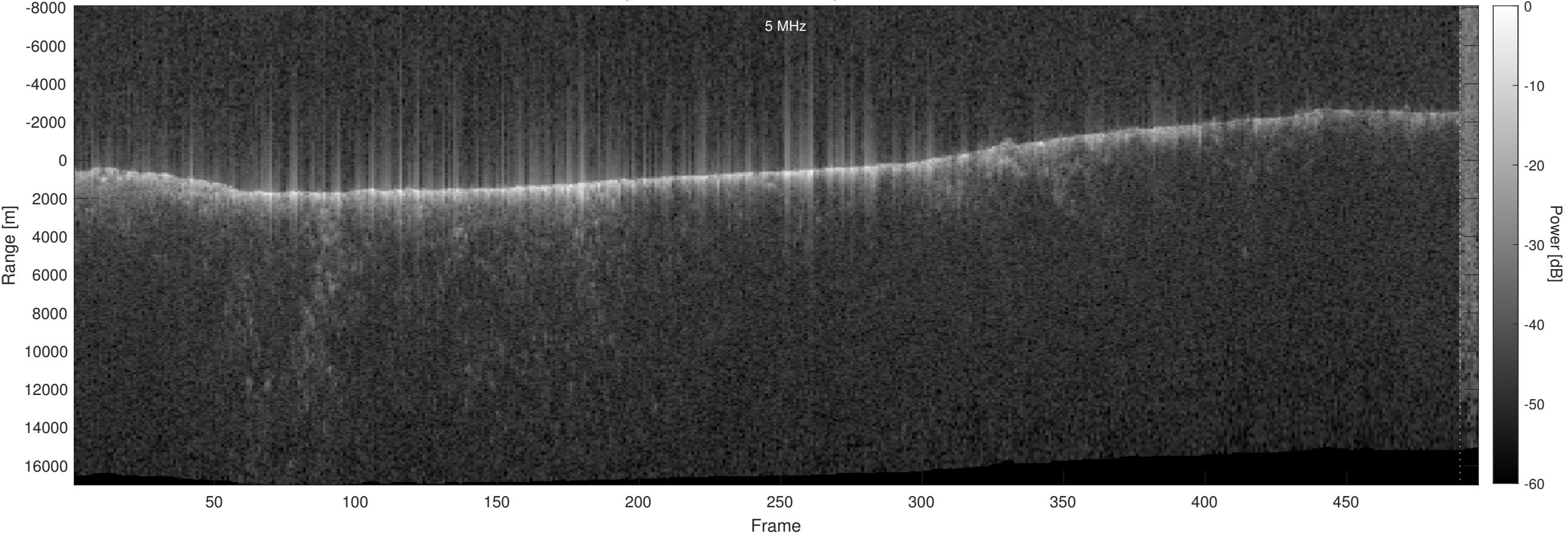
Orbit 16010, Optimized, No Window, Depth-Corrected, Channel 2
