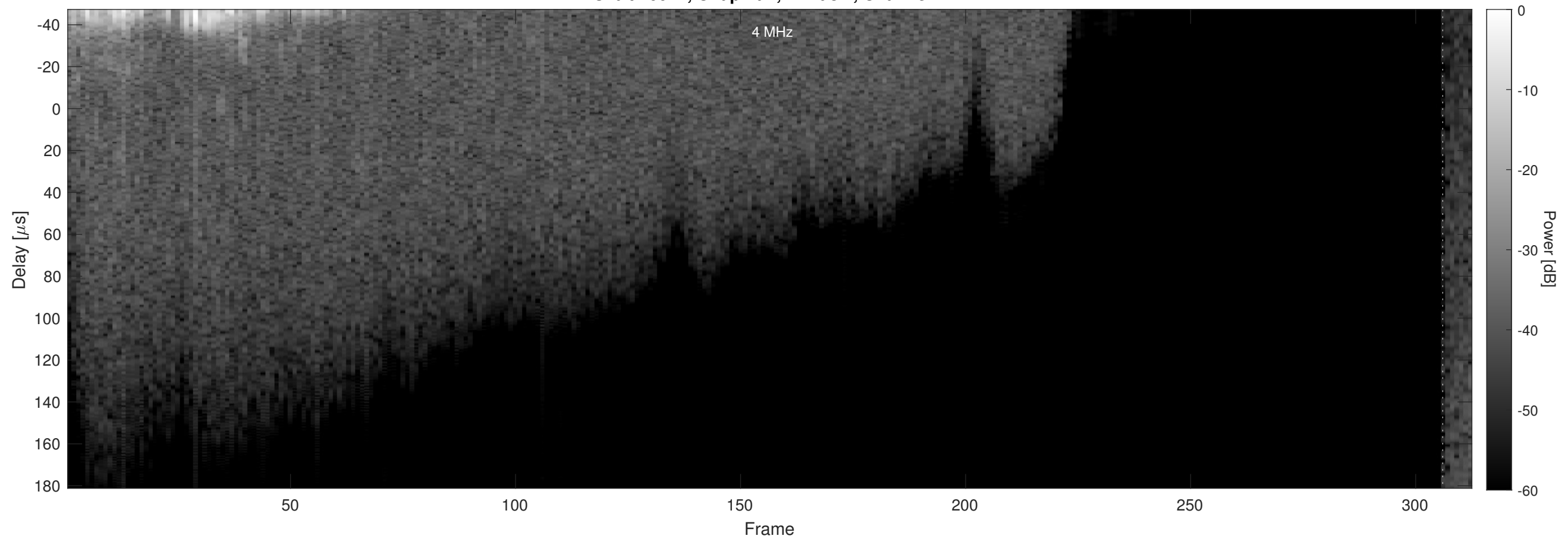
Orbit 16011, Chapman, Window, Channel 2
