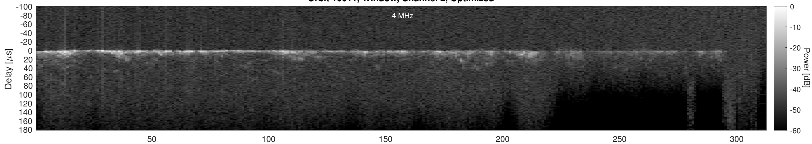
Orbit 16011, Cluttergram
