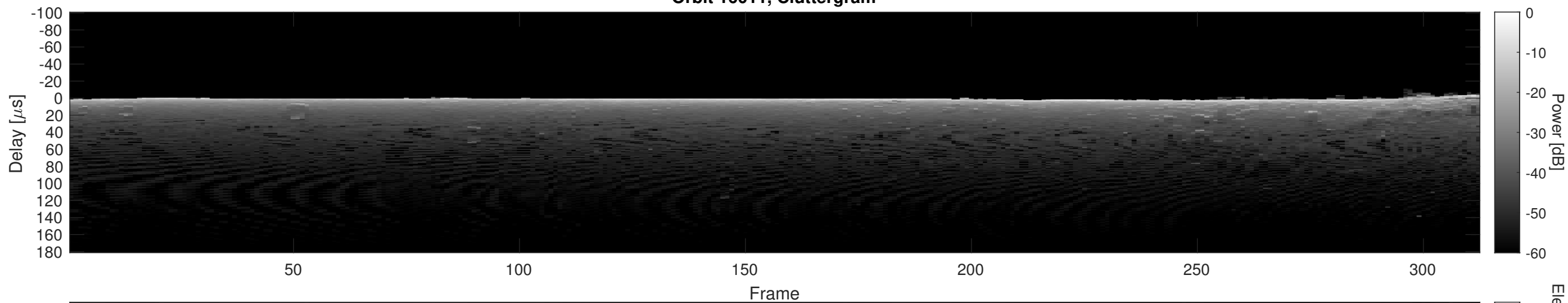
Orbit 16011, Cluttergram
