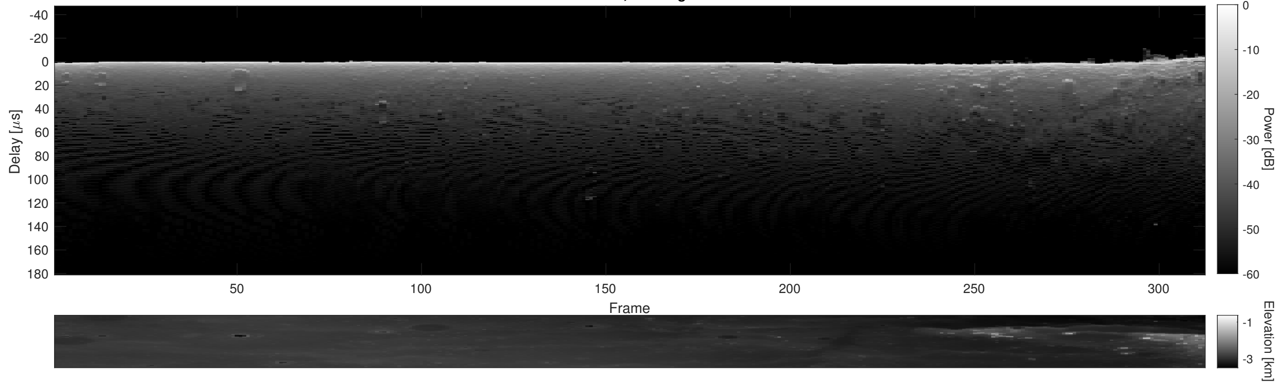
Orbit 16011, Cluttergram
