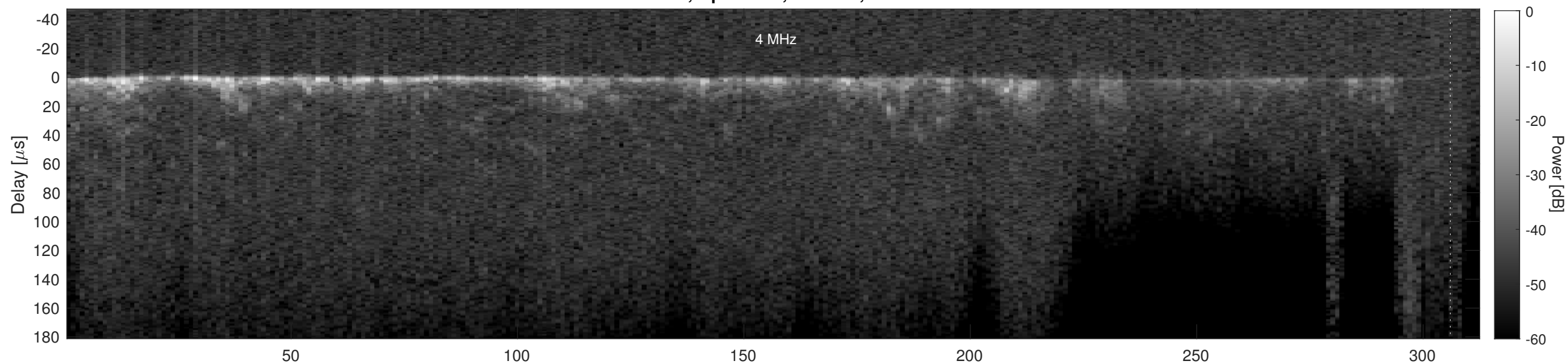
Orbit 16011, Cluttergram
