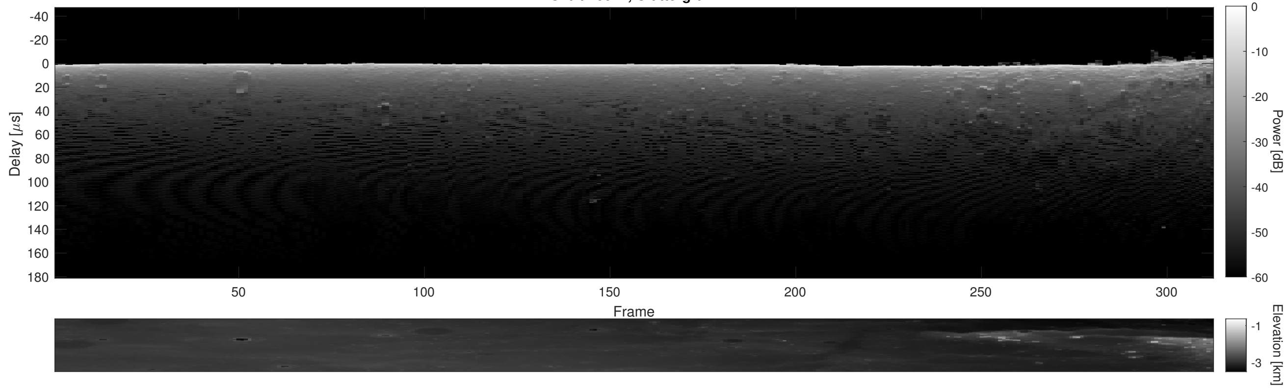
Orbit 16011, Cluttergram
