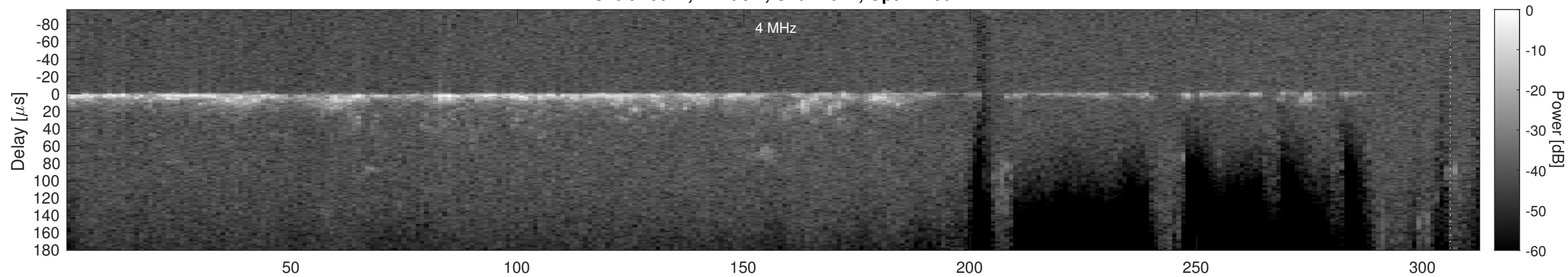
Orbit 16012, Cluttergram
