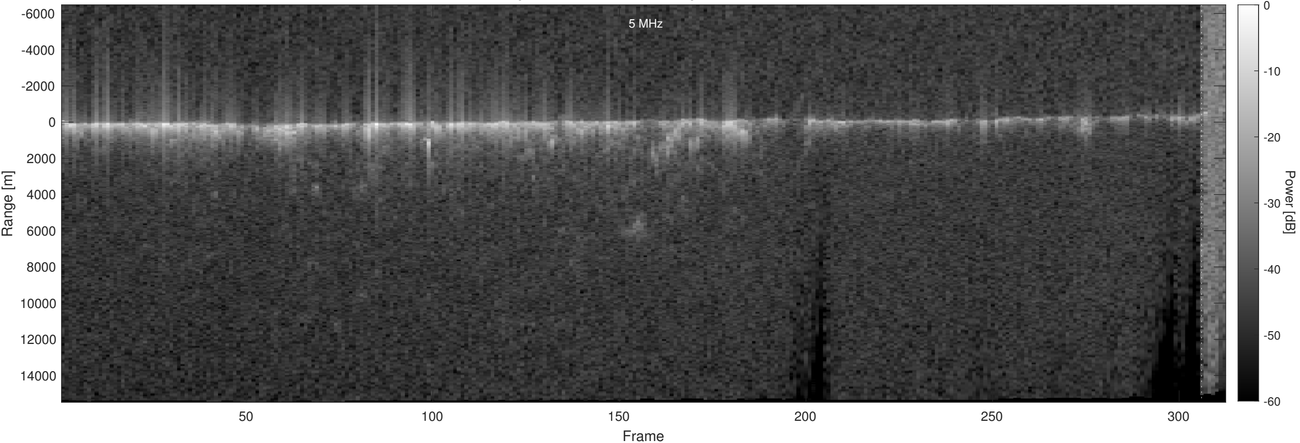
Orbit 16012, Optimized, No Window, Depth-Corrected, Channel 2
