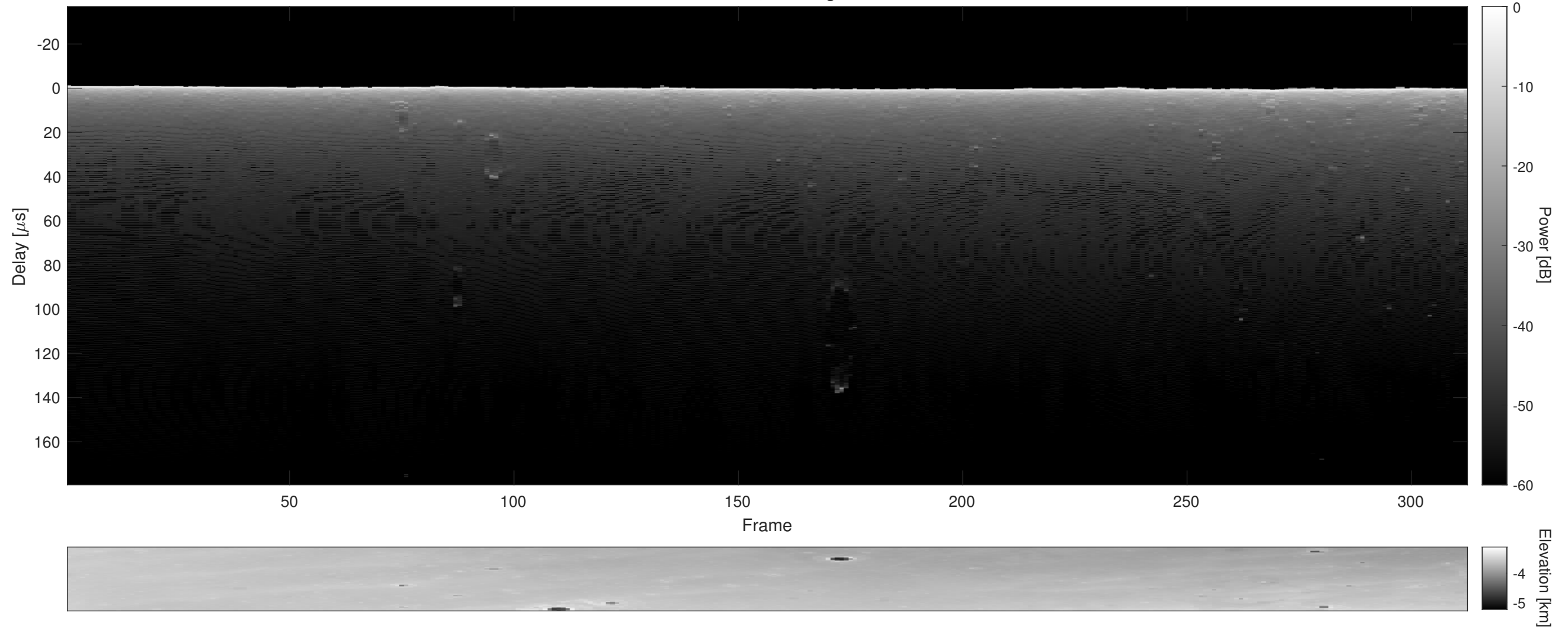
Orbit 16013, Cluttergram
