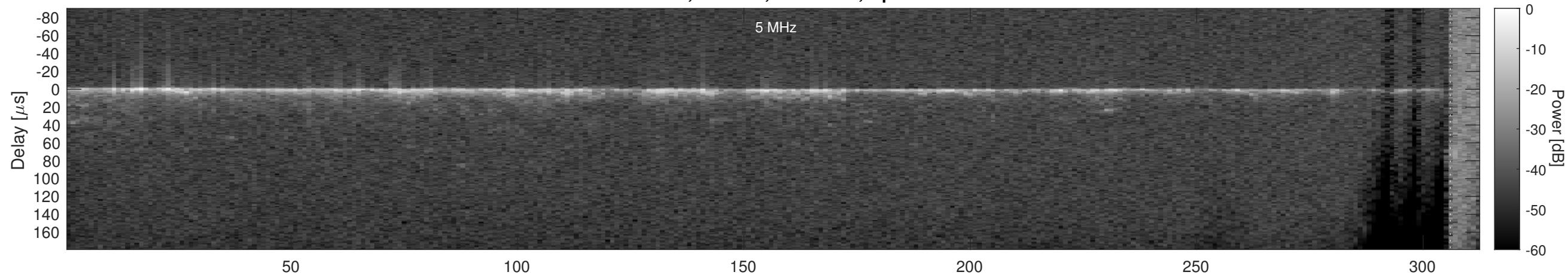
Orbit 16013, Cluttergram
