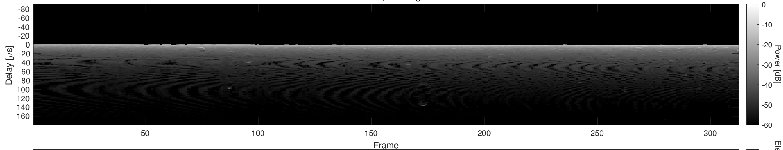
Orbit 16013, Cluttergram
