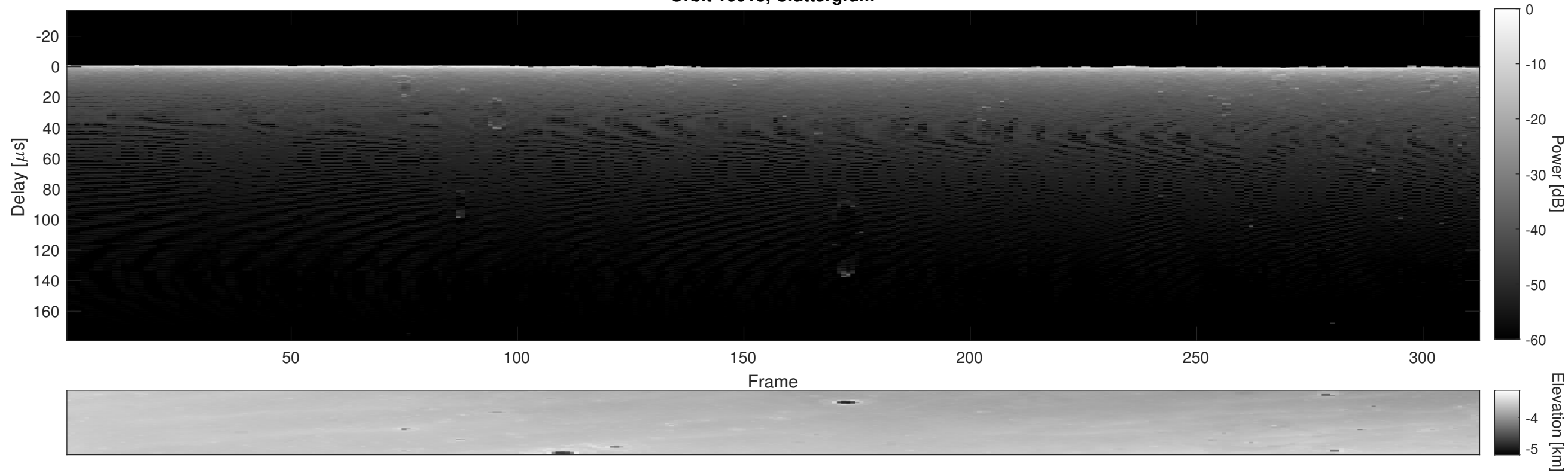
Orbit 16013, Cluttergram
