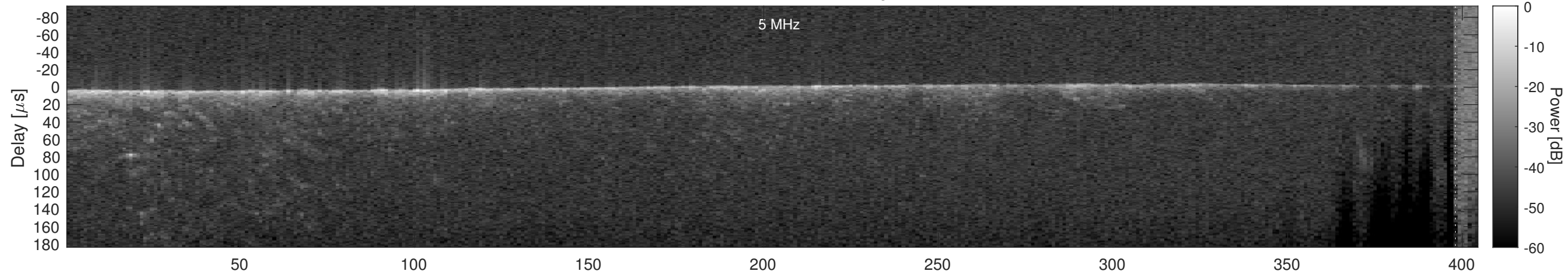
Orbit 16014, Cluttergram
