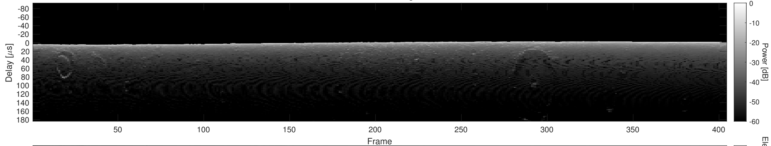
Orbit 16014, Cluttergram
