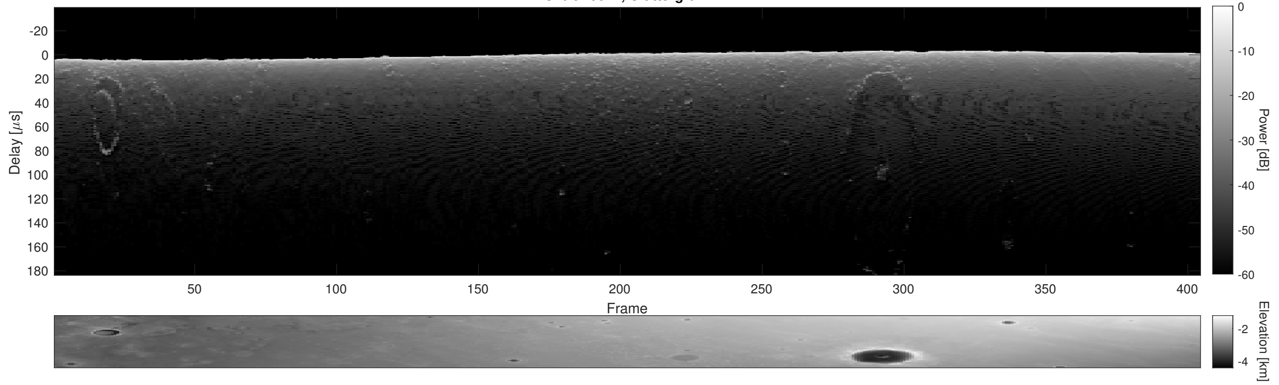
Orbit 16014, Cluttergram
