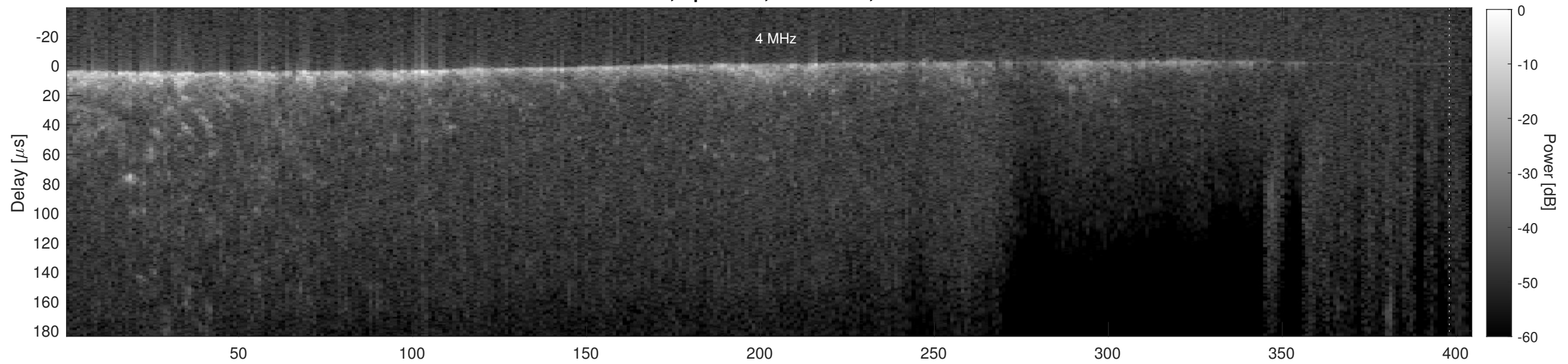
Orbit 16014, Cluttergram
