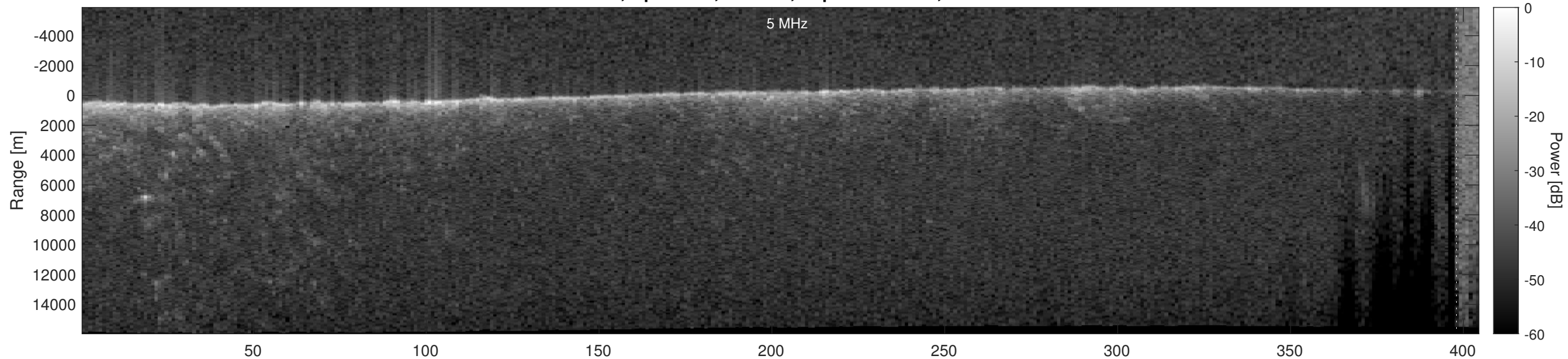
Orbit 16014, Optimized, Window, Depth-Corrected, Channel 2
