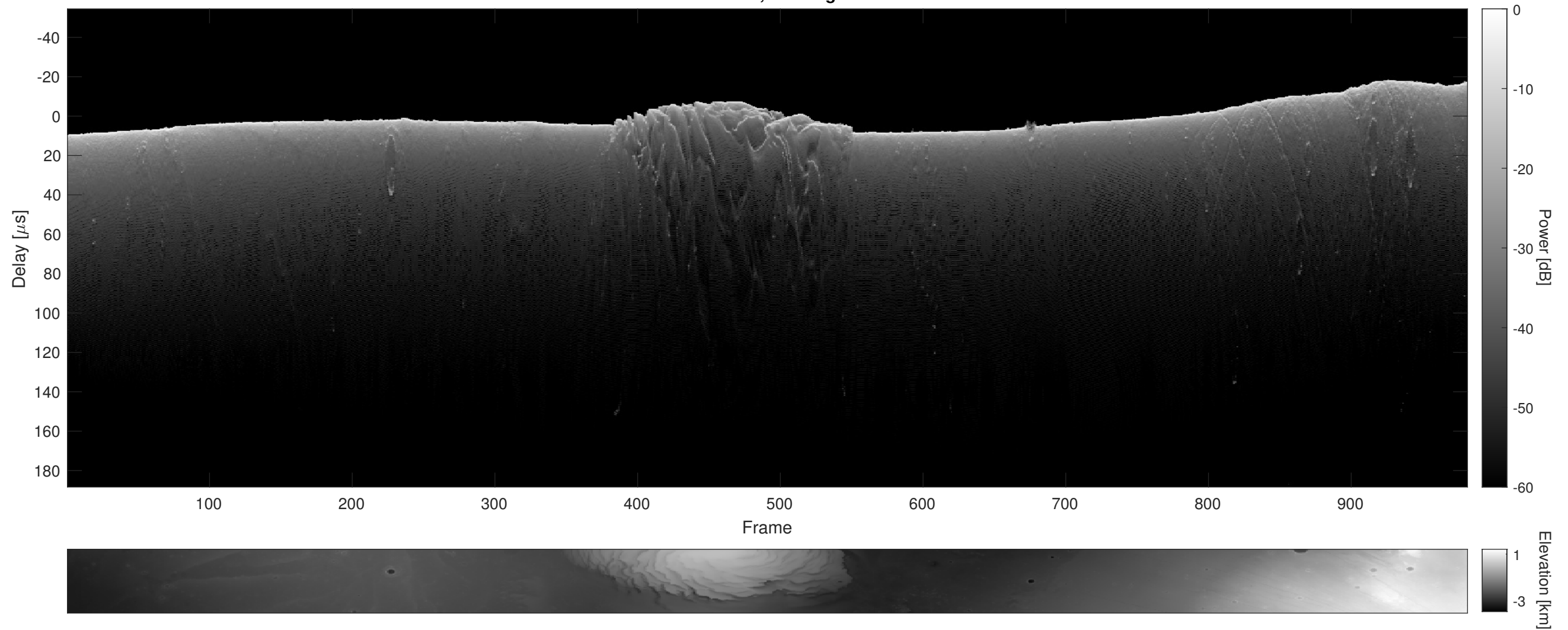
Orbit 16017, Cluttergram
