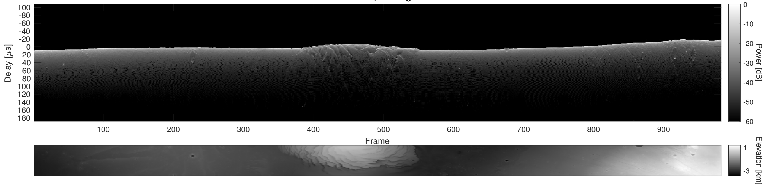
Orbit 16017, Cluttergram
