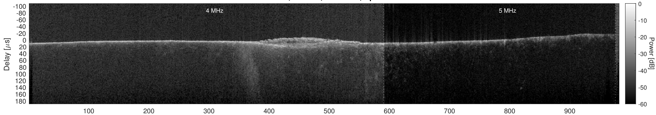
Orbit 16017, Cluttergram
