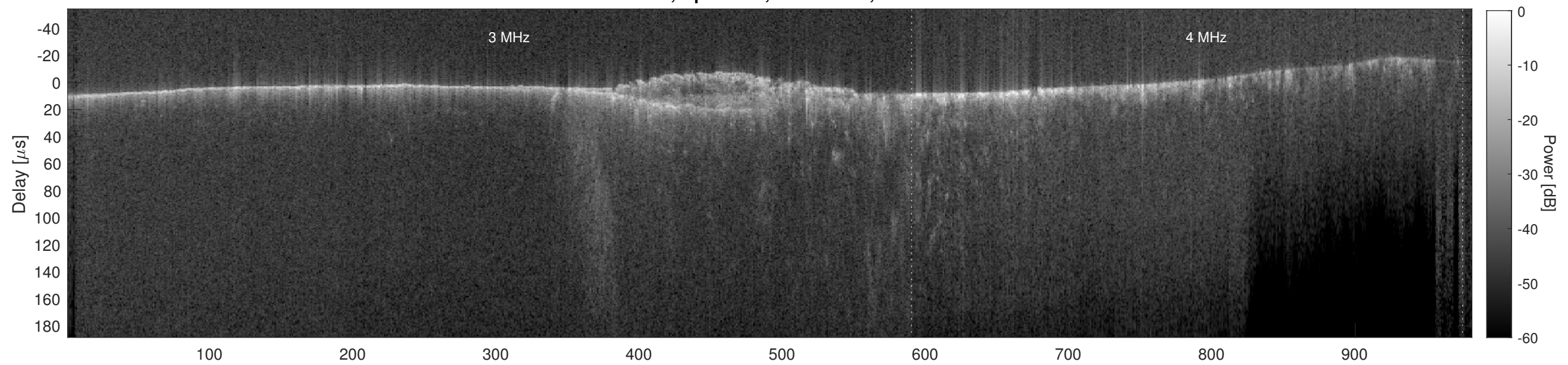
Orbit 16017, Cluttergram
