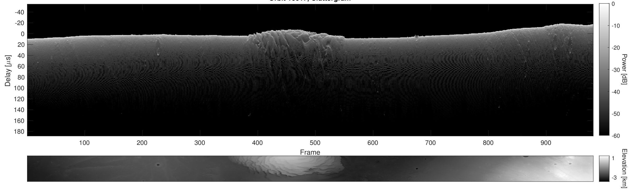
Orbit 16017, Cluttergram
