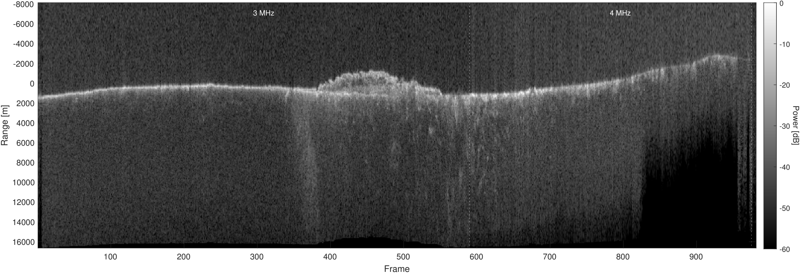
Orbit 16017, Optimized, Window, Depth-Corrected, Channel 2
