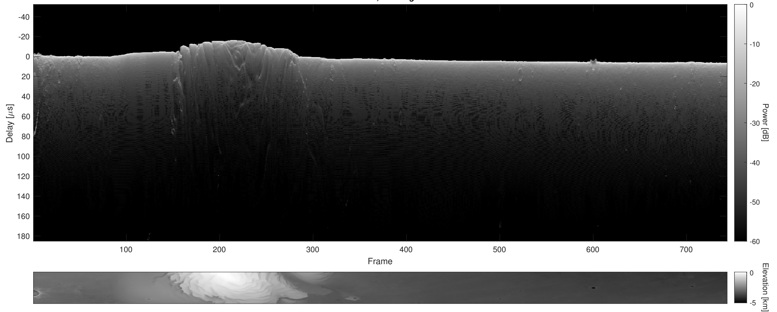
Orbit 16020, Cluttergram
