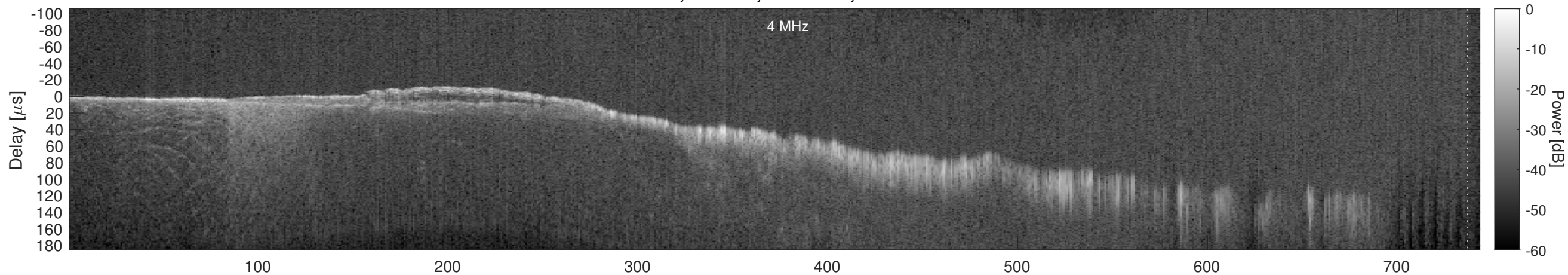
Orbit 16020, Window, Channel 2, Chapman
