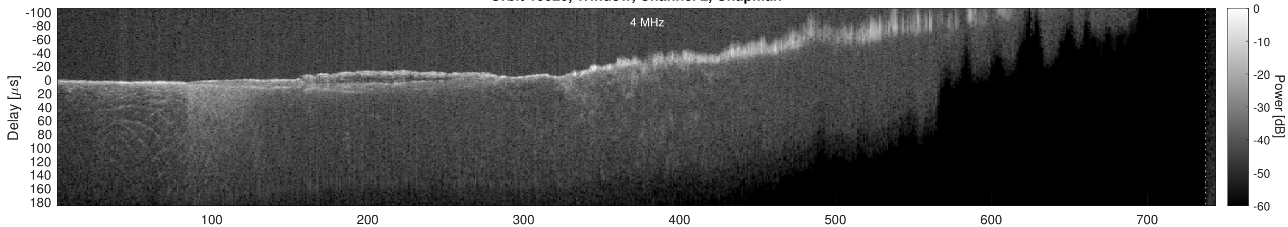
Orbit 16020, Window, Channel 2, Optimized
