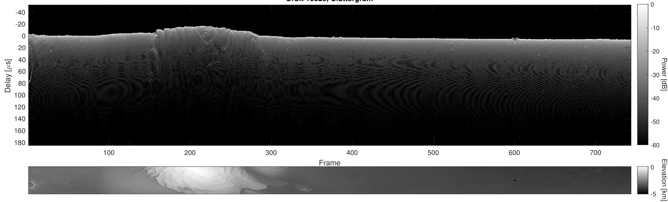
Orbit 16020, Cluttergram
