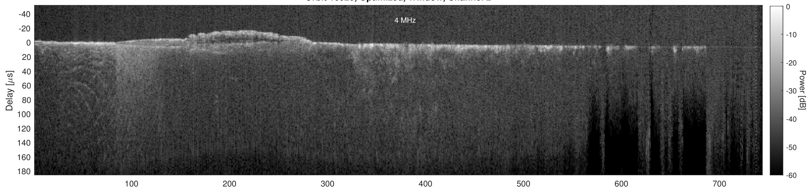
Orbit 16020, Cluttergram
