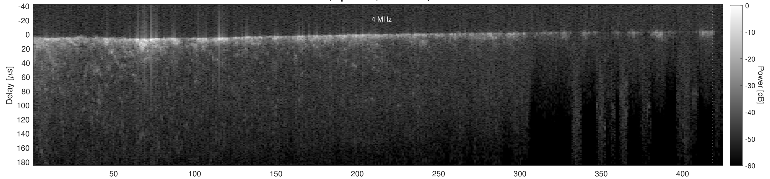
Orbit 16021, Cluttergram
