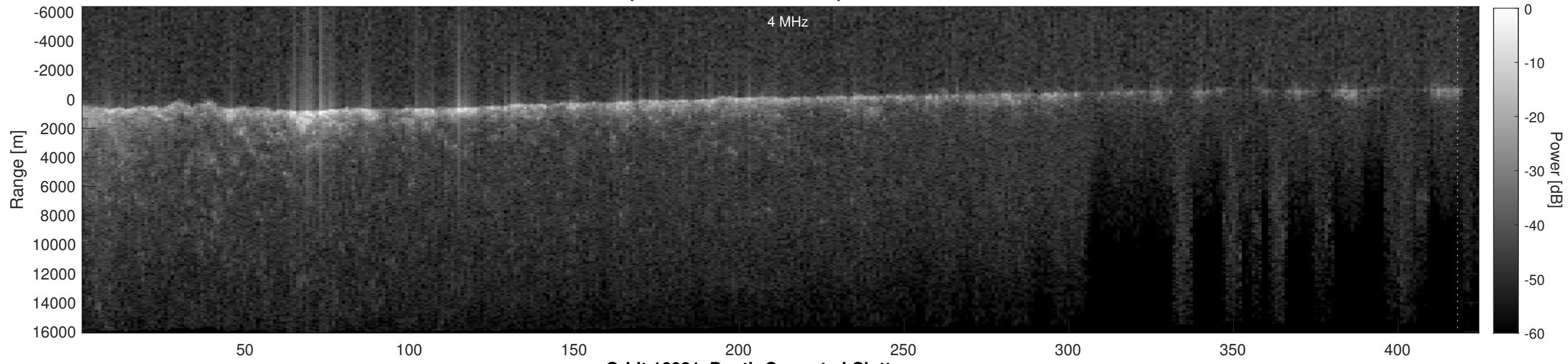
Orbit 16021, Depth-Corrected Cluttergram
