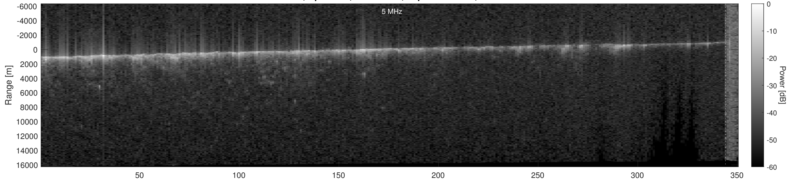
Orbit 16028, Optimized, No Window, Depth-Corrected, Channel 2
