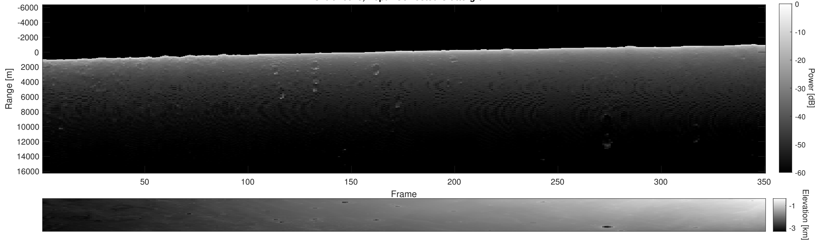
Orbit 16028, Depth-Corrected Cluttergram
