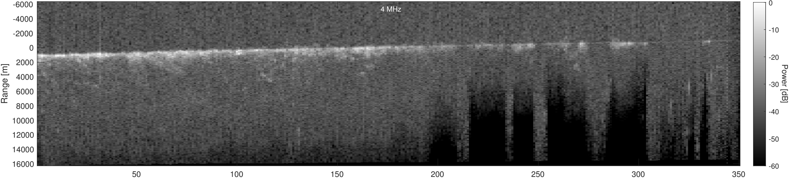
Orbit 16028, Depth-Corrected Cluttergram
