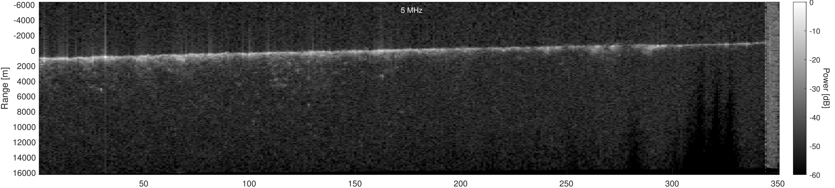
Orbit 16028, Optimized, Window, Depth-Corrected, Channel 2
