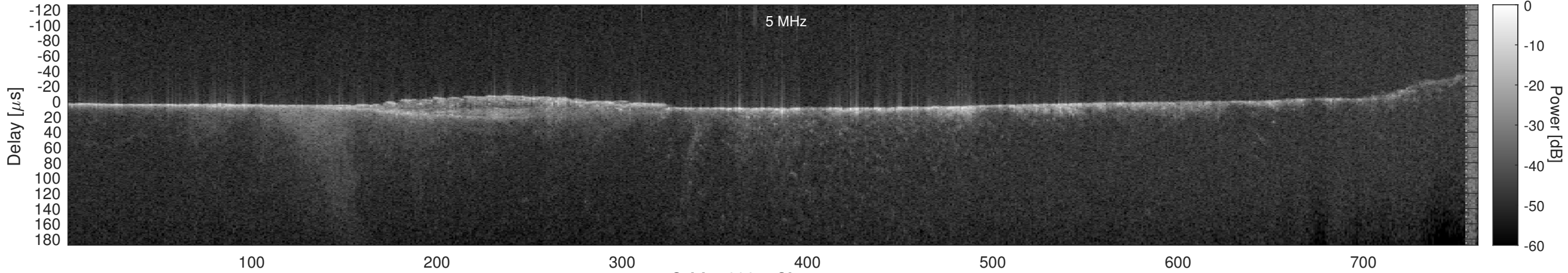
Orbit 16031, Cluttergram
