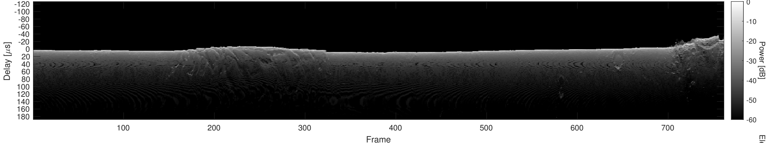
Orbit 16031, Cluttergram
