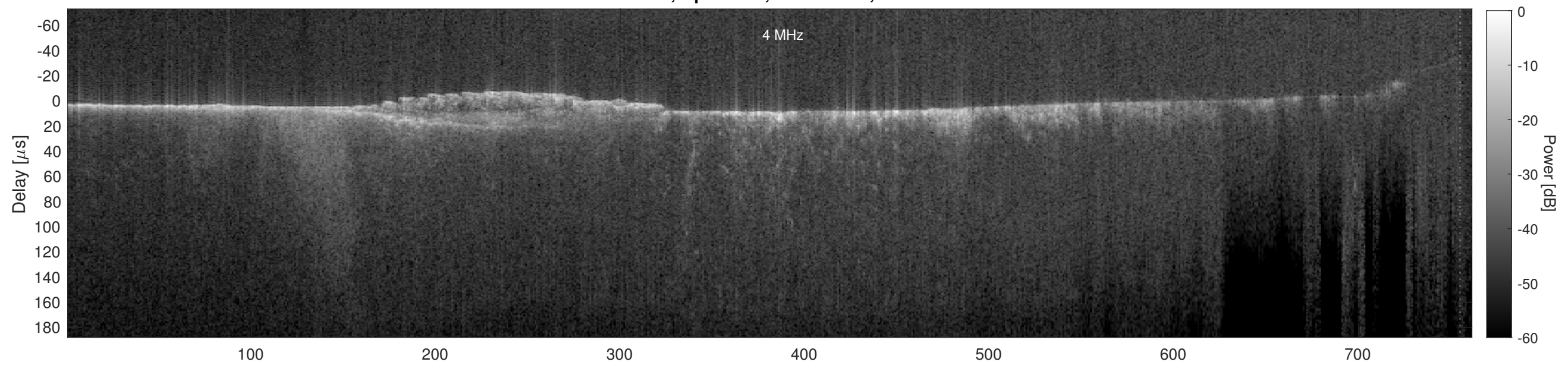
Orbit 16031, Cluttergram
