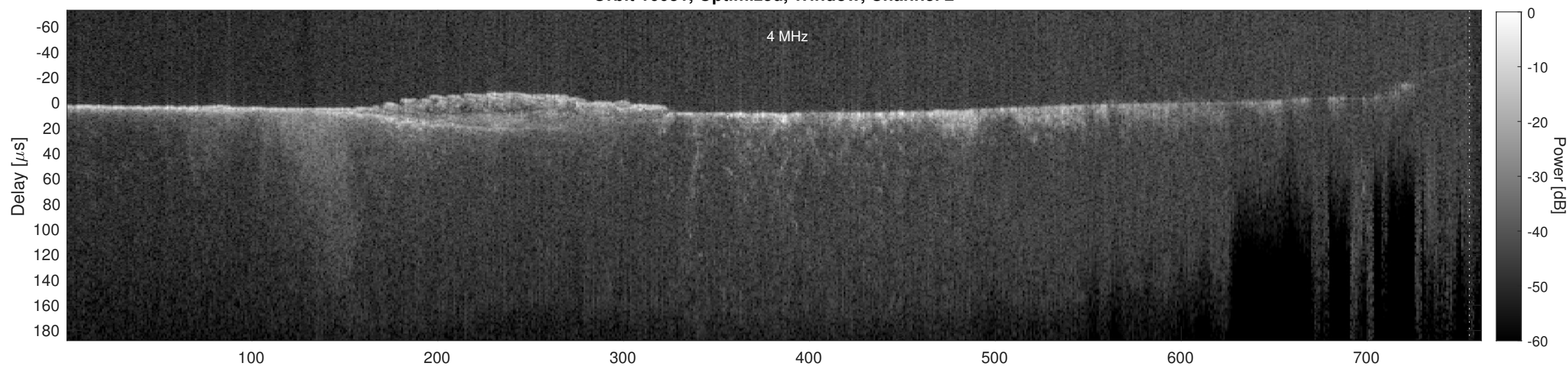
Orbit 16031, Cluttergram
