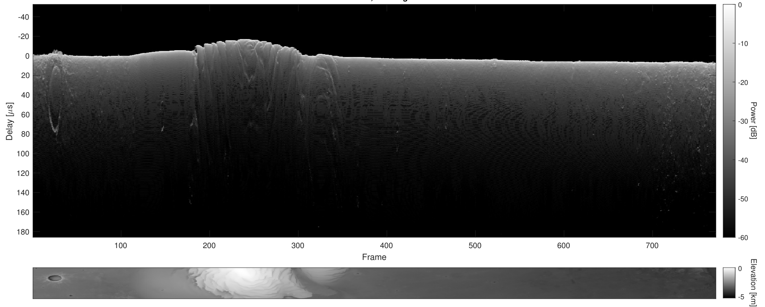
Orbit 16034, Cluttergram
