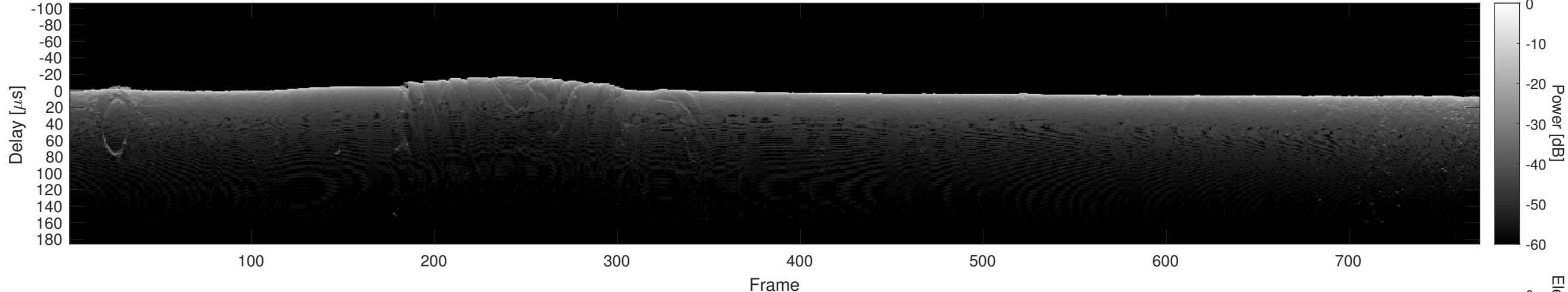
Orbit 16034, Cluttergram
