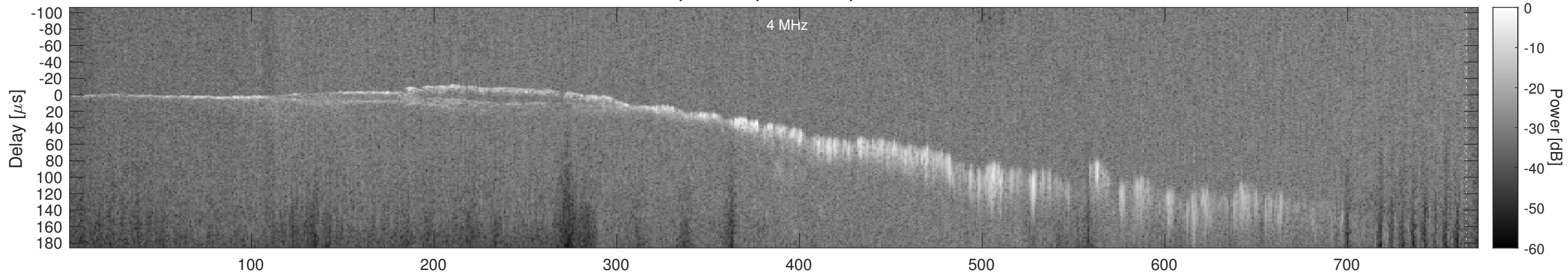
Orbit 16034, Window, Channel 2, Chapman
