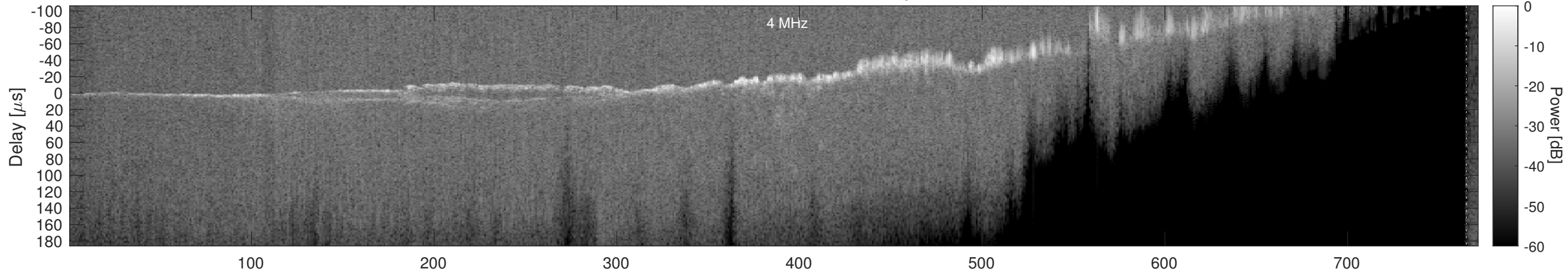
Orbit 16034, Window, Channel 2, Optimized
