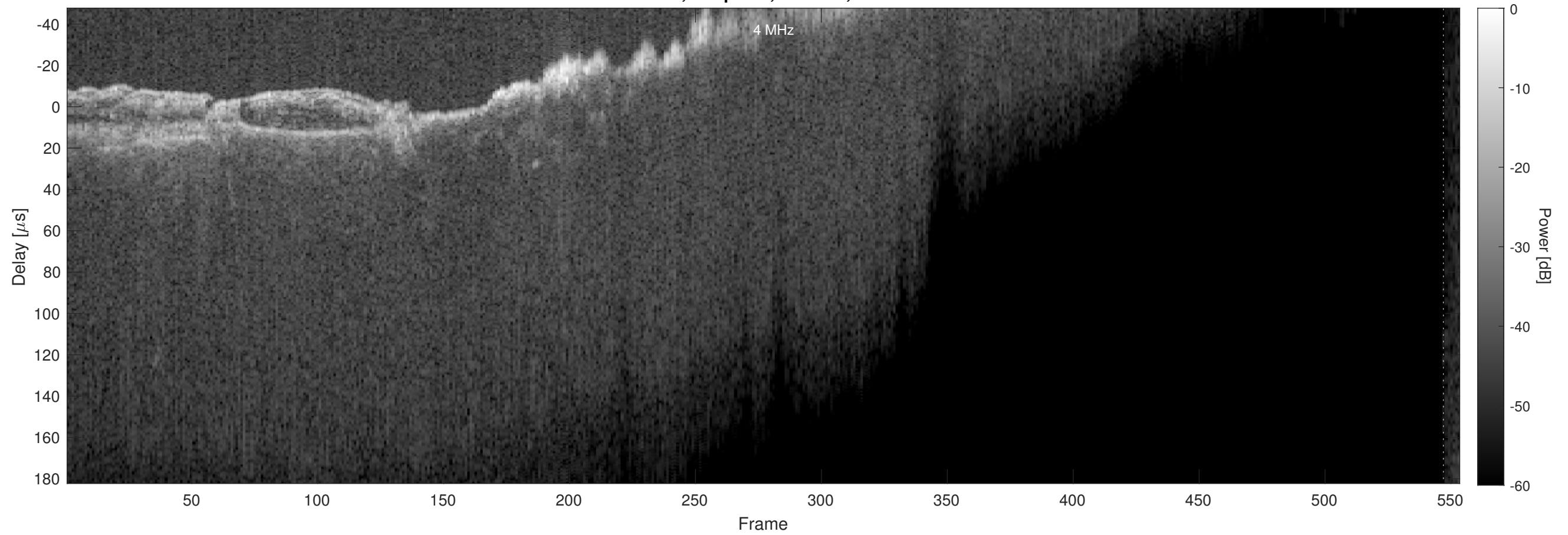
Orbit 16037, Chapman, Window, Channel 2
