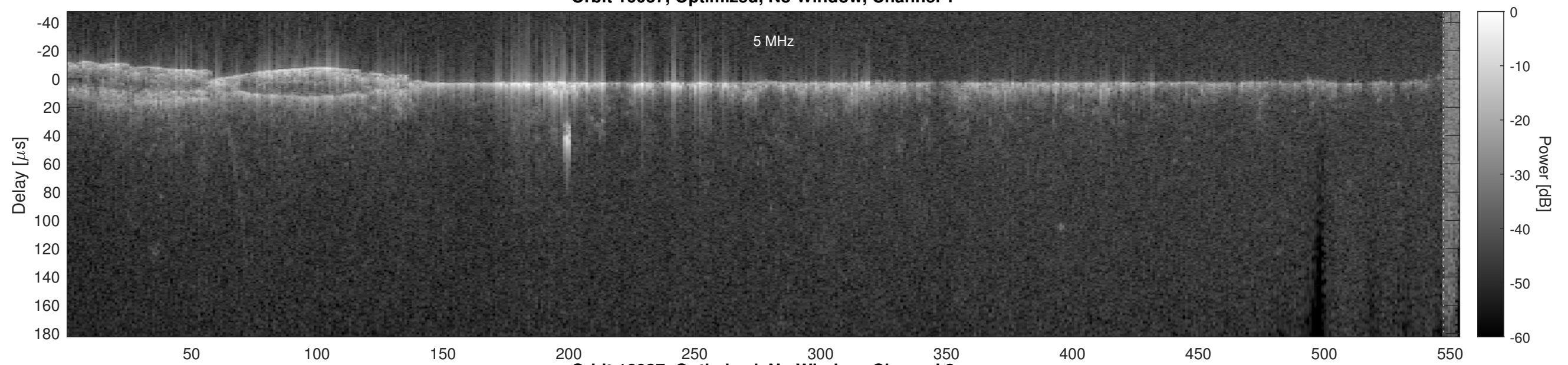
Orbit 16037, Optimized, No Window, Channel 2
