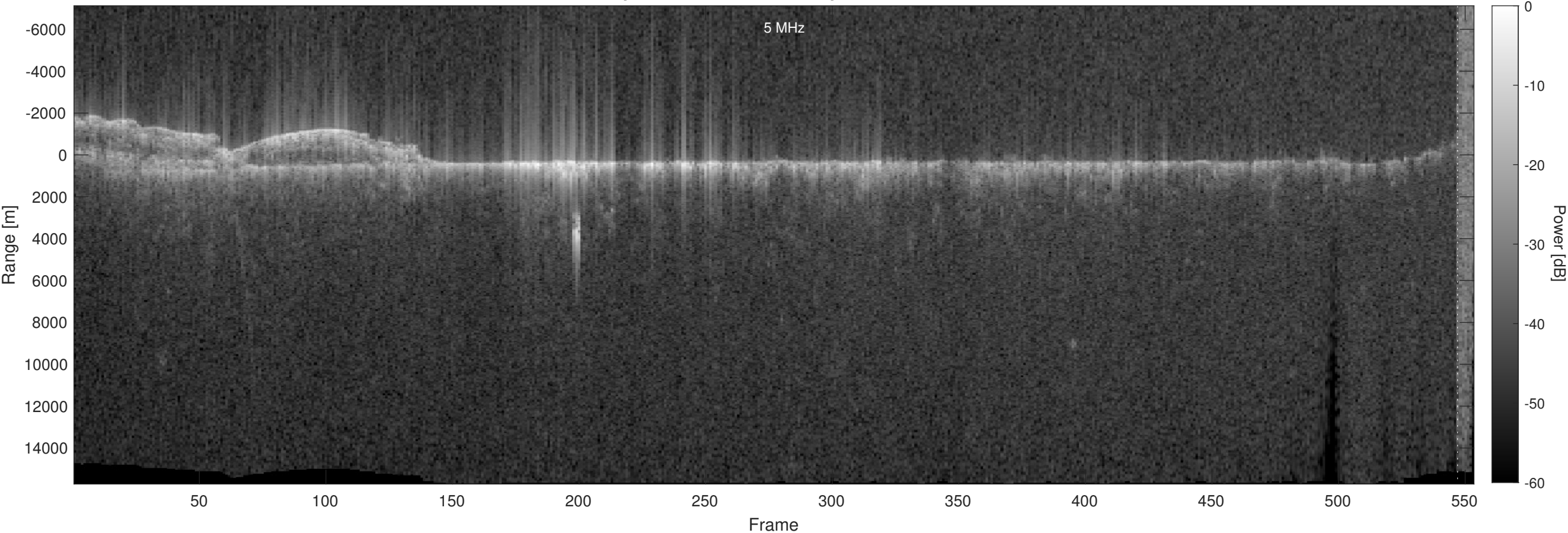
Orbit 16037, Optimized, No Window, Depth-Corrected, Channel 2
