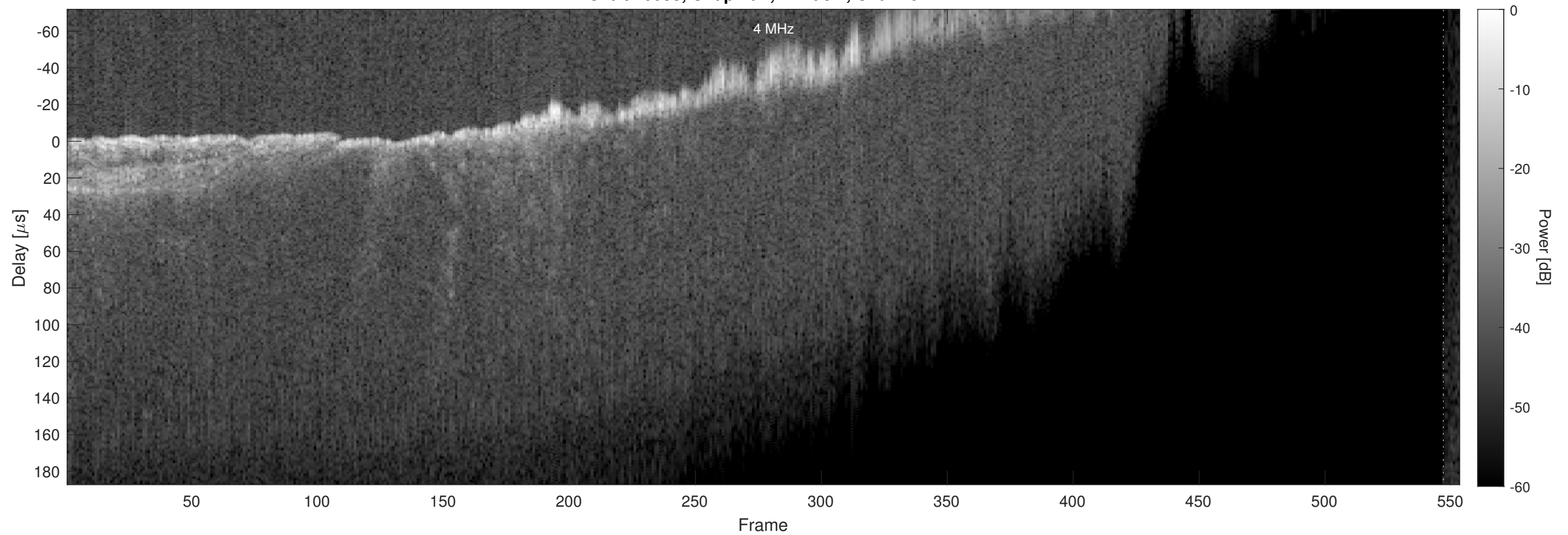
Orbit 16038, Chapman, Window, Channel 2
