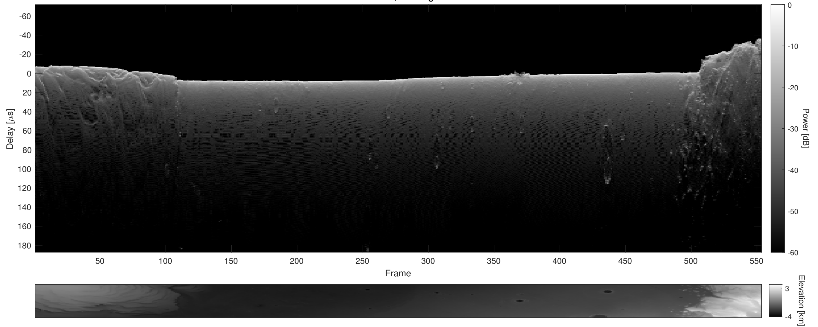
Orbit 16038, Cluttergram
