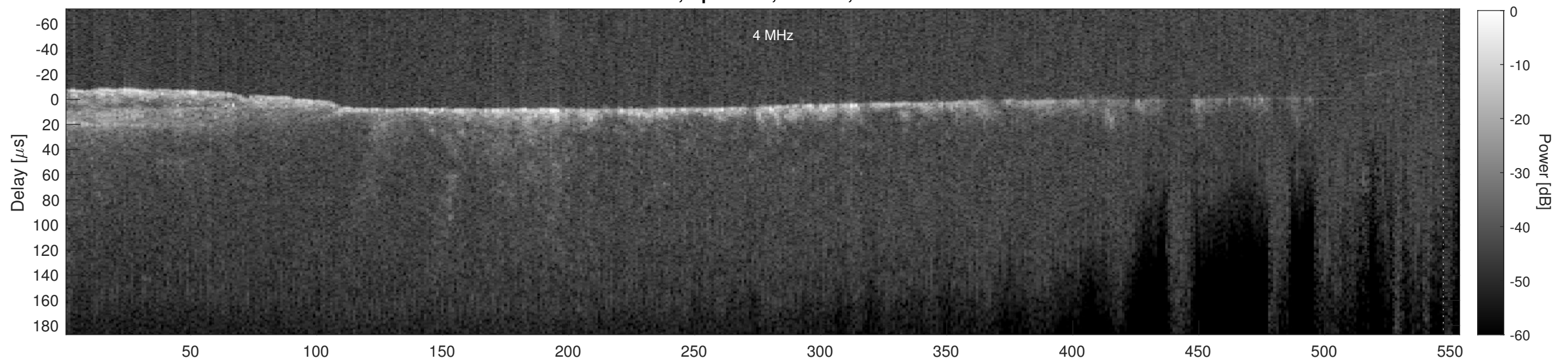
Orbit 16038, Cluttergram
