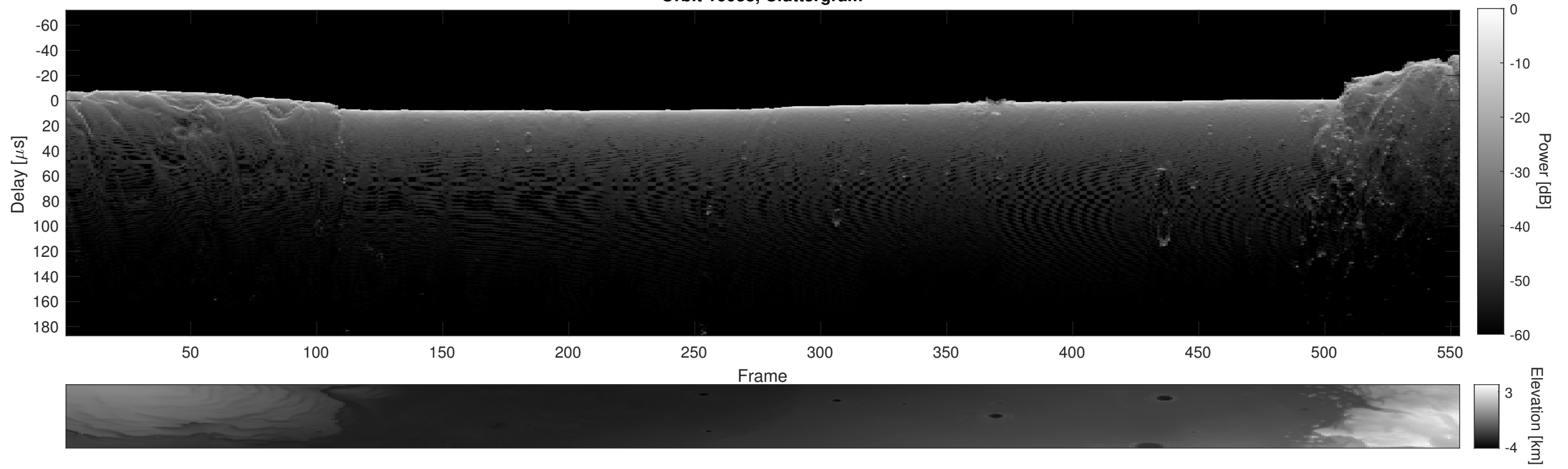
Orbit 16038, Cluttergram
