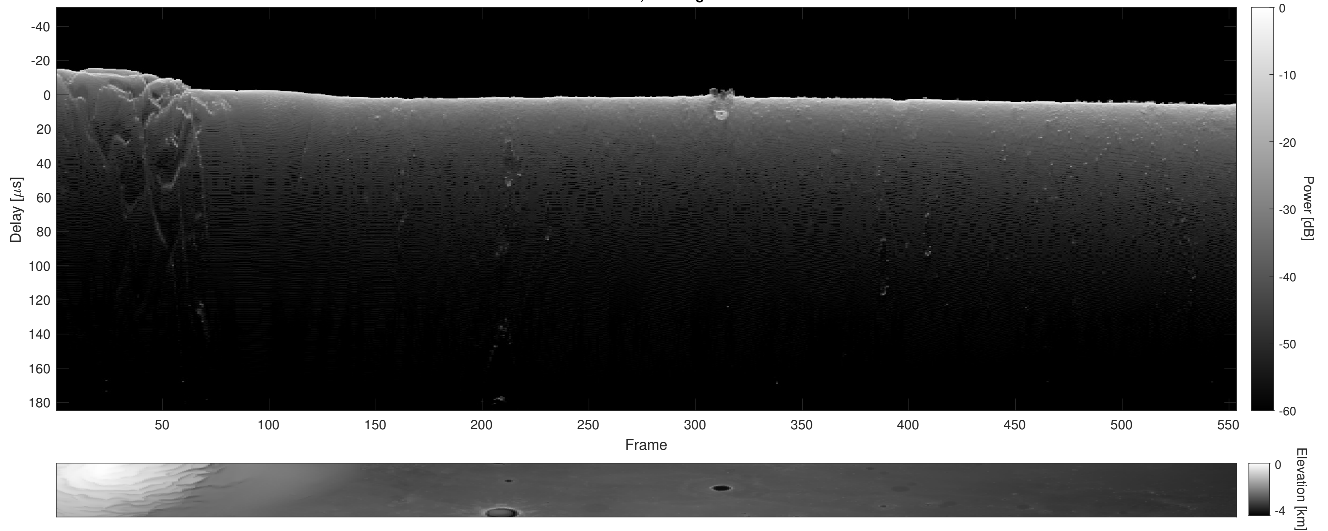
Orbit 16039, Cluttergram
