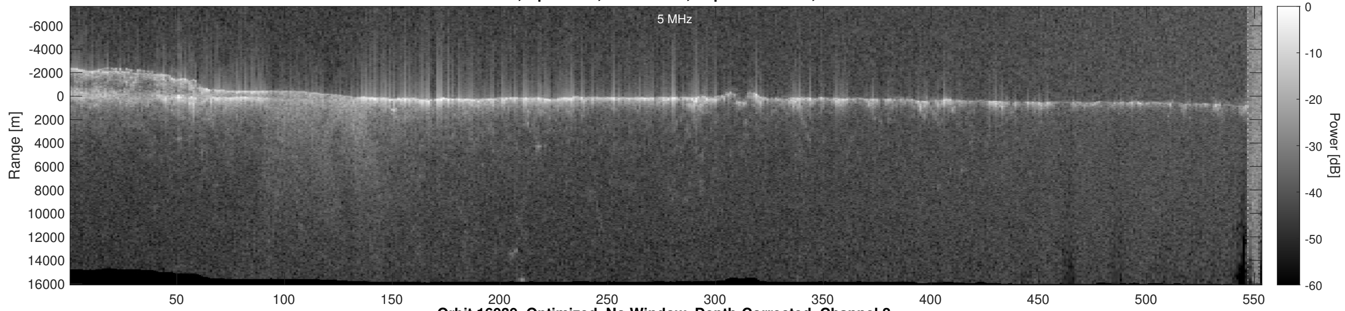
Orbit 16039, Optimized, No Window, Depth-Corrected, Channel 2
