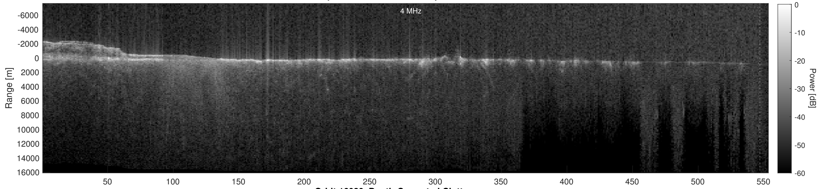
Orbit 16039, Depth-Corrected Cluttergram
