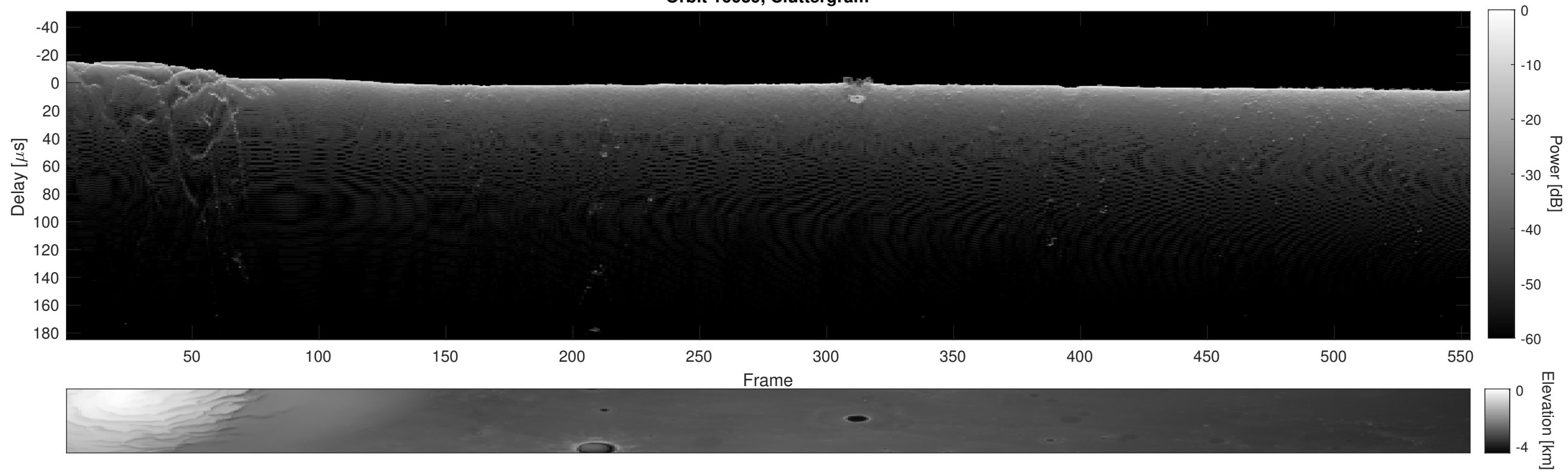
Orbit 16039, Cluttergram
