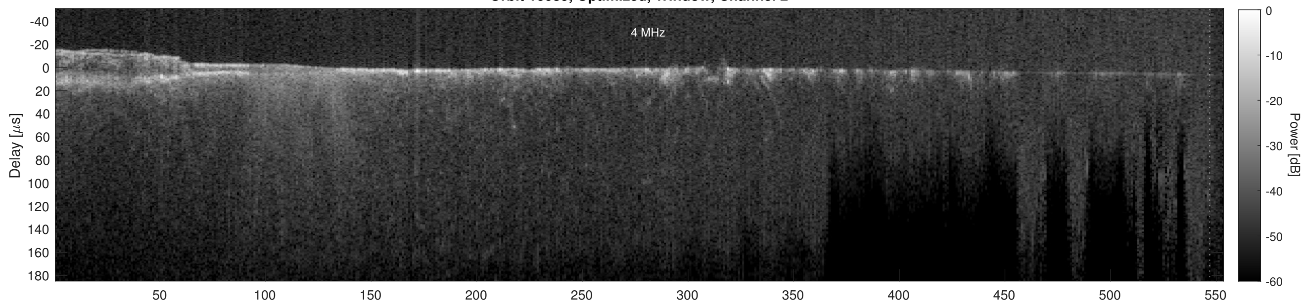
Orbit 16039, Cluttergram
