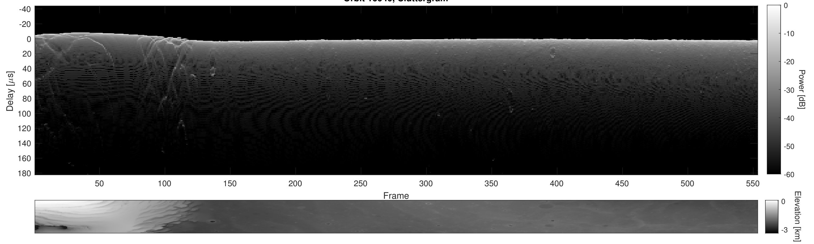
Orbit 16040, Cluttergram
