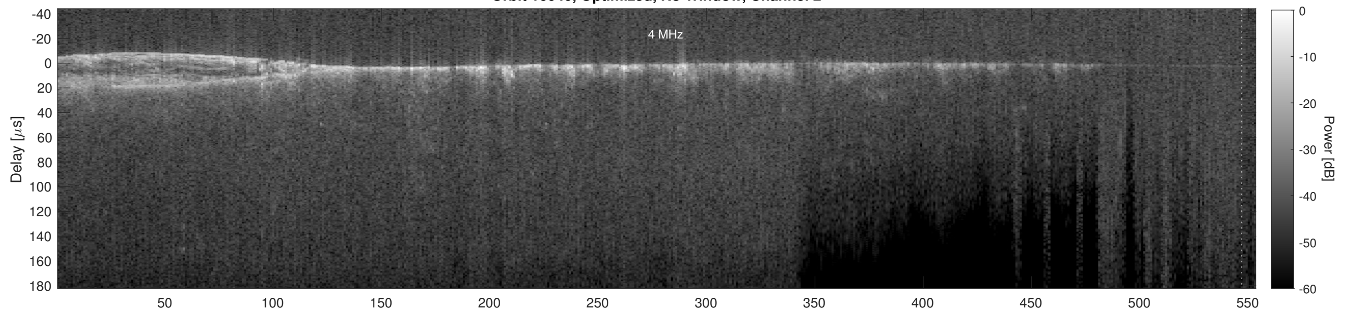
Orbit 16040, Cluttergram
