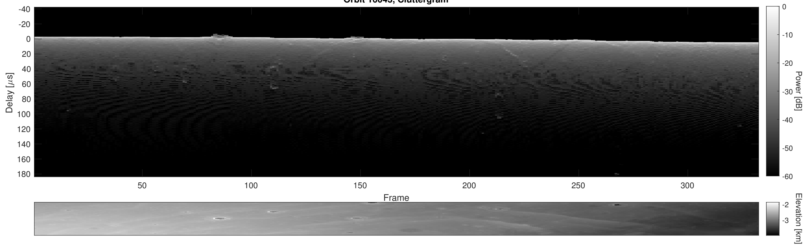
Orbit 16043, Cluttergram
