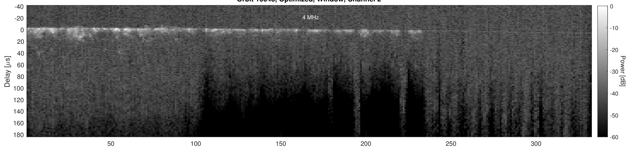
Orbit 16043, Cluttergram
