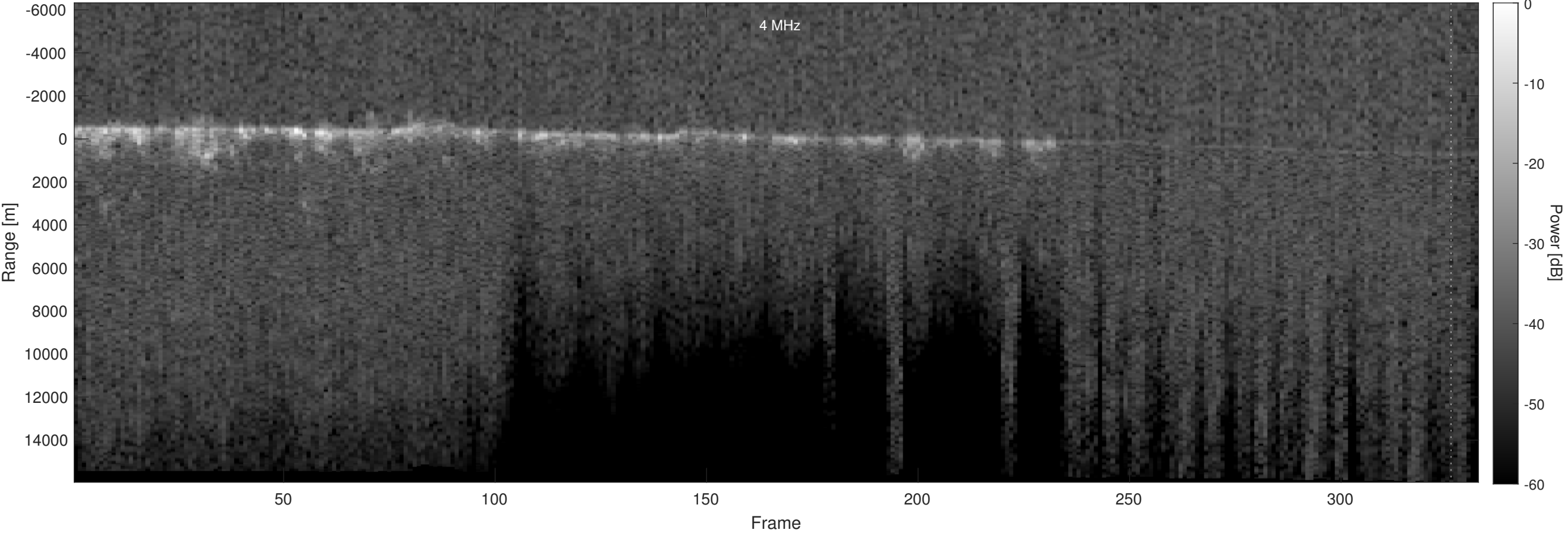
Orbit 16043, Optimized, Window, Depth-Corrected, Channel 2
