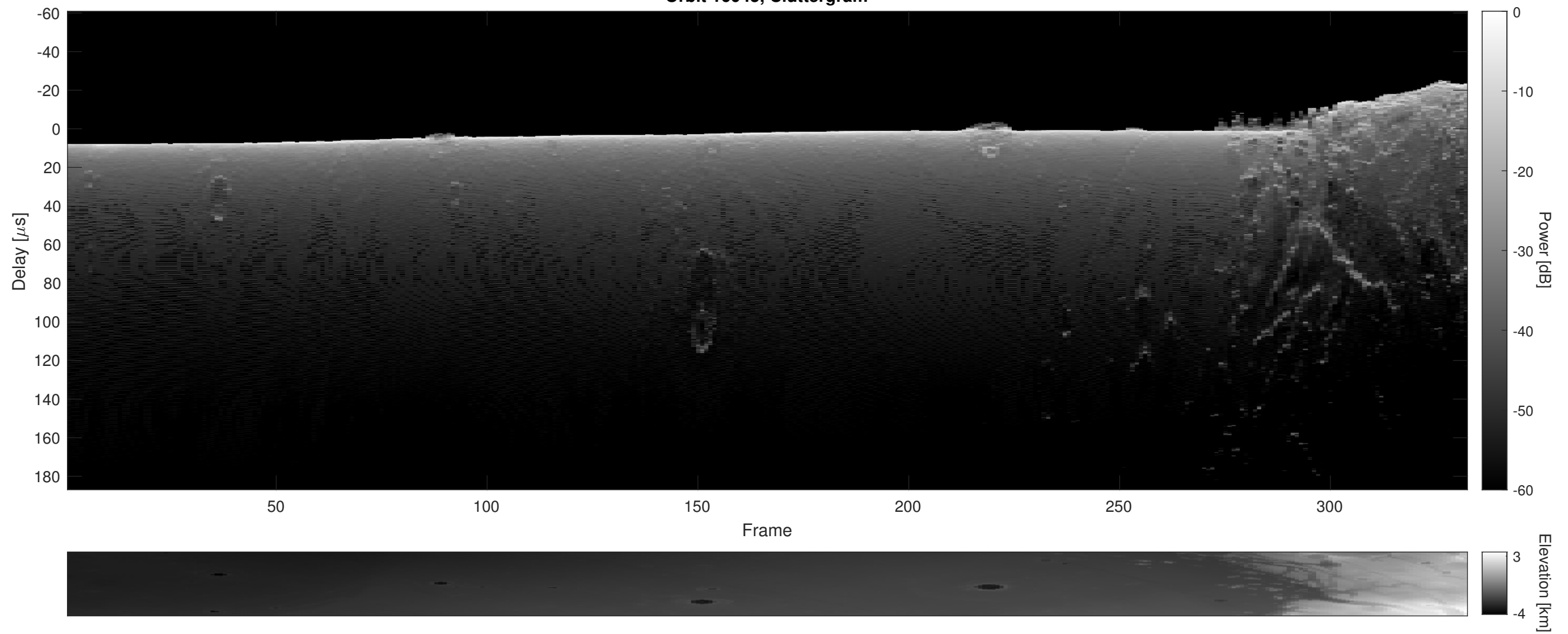
Orbit 16045, Cluttergram
