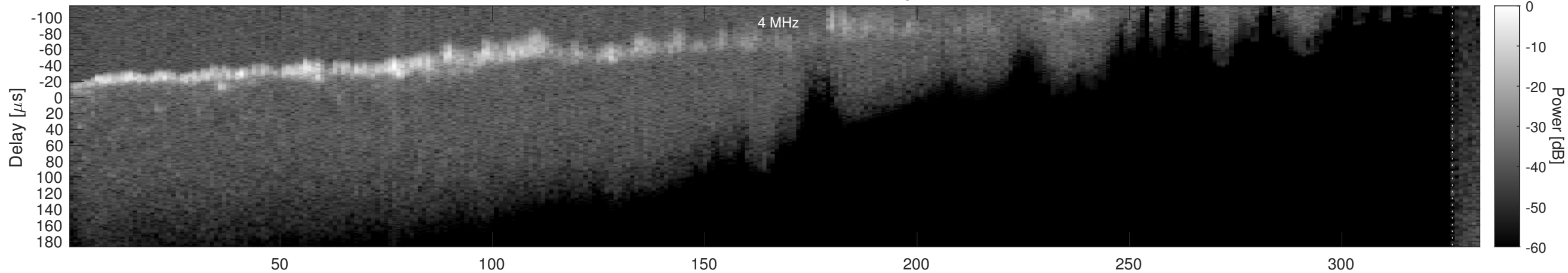
Orbit 16045, Window, Channel 2, Optimized
