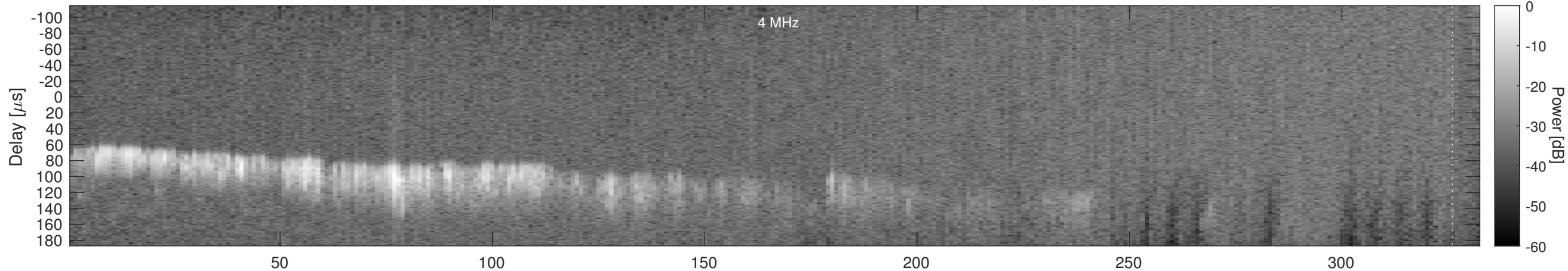
Orbit 16045, Window, Channel 2, Chapman
