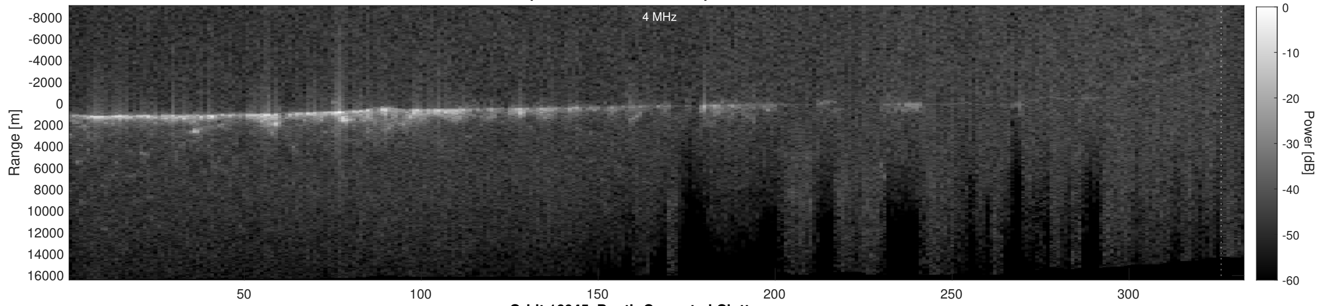
Orbit 16045, Depth-Corrected Cluttergram
