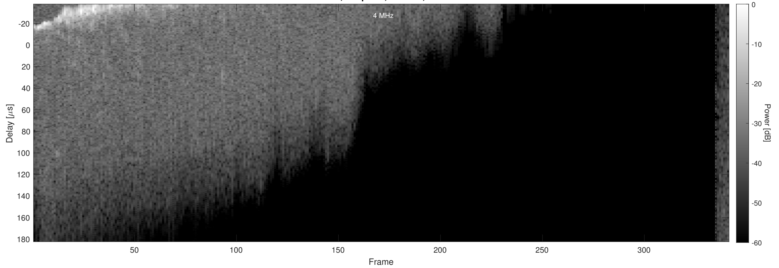
Orbit 16046, Chapman, Window, Channel 2
